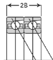
DT Tandem Arrangement
