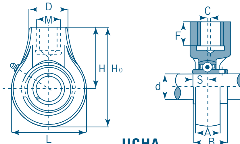
UCHA Set Screw Locking
